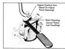
Fig. 12-48 Checking and Adjusting Voltage Regulator Point Opening
