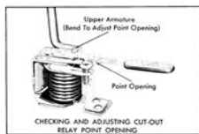
Fig. 12-43 Checking and Adjusting Cut-Out Relay Point Opening
