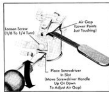
Fig. 12-47 Checking and Adjusting Voltage Regulator Air Gap
