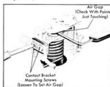
Fig. 12-46 Checking and Adjusting Current Regulator Air Gap
